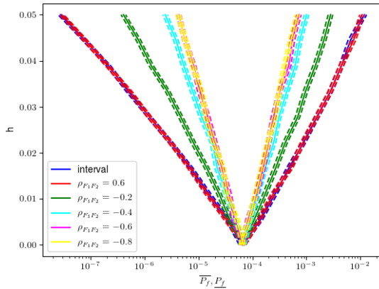
Figure 9: G_2 comparison of robustness and opportuneness curves for toy case 2.
